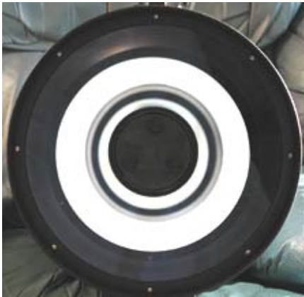
Figure 1. Mirror pattern of collimated scope.
